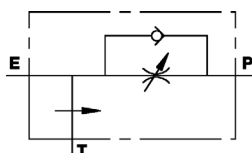
VALVOLA PRIORITARIA A 3 VIE - RFP3
